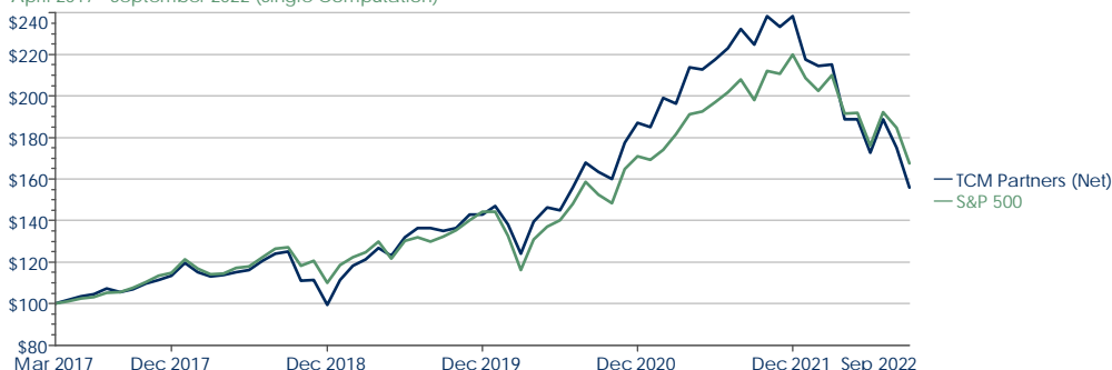
TCM Partners Strategy Performance April 2017 - September 2022 (Single Computation)
